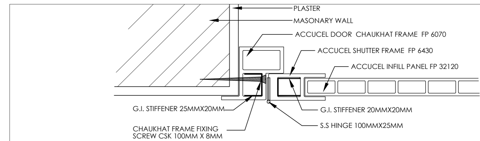
SECTION X
